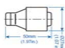
FUSIBLE DIAZED DZ3 ACCION LENTA
