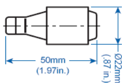
FUSIBLE DIAZED DZ2 ACCION RAPIDA
